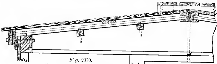
Fig. 2370. Part Cross-section of Roof.
